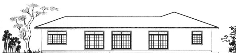
FRONT ELEVATION
